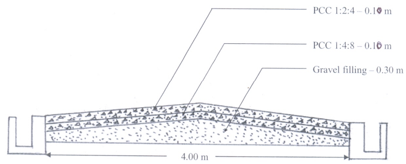
Cross section for Road work
