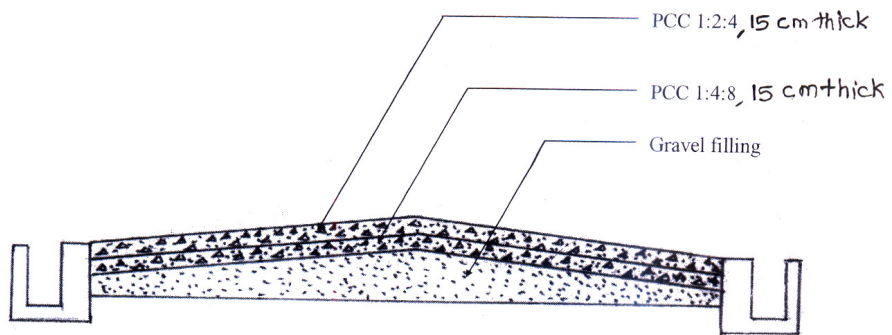
Cross section for Road work
