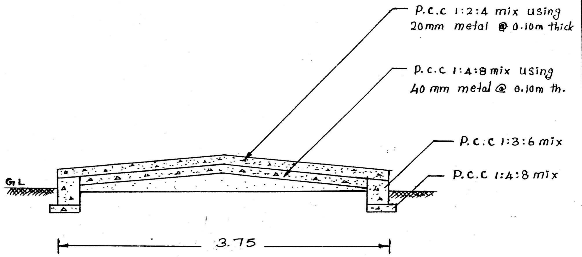
Cross Section for Road
