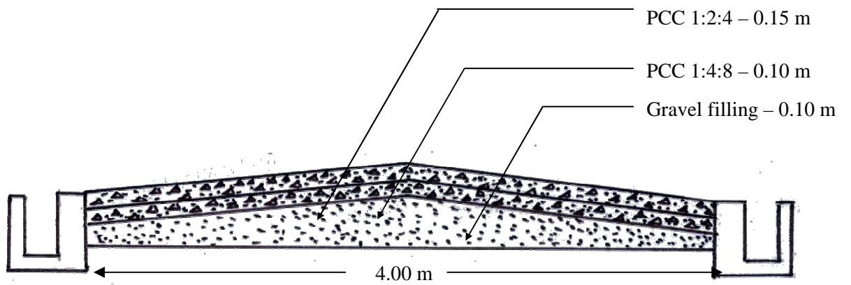
Cross section for Road work
