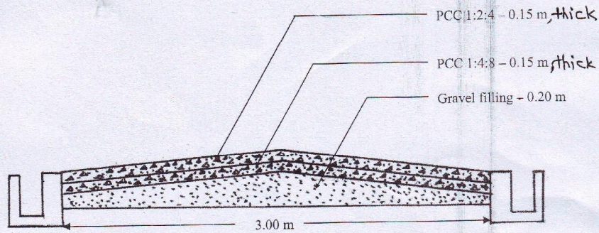
Cross section for Road work
