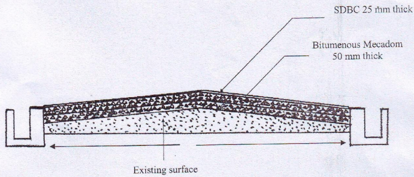
Cross section for Road work
