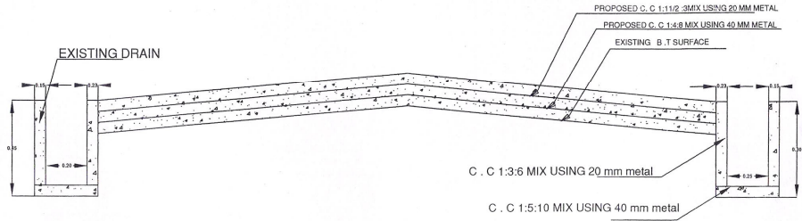
CROSS SECTION OF C. C ROAD
