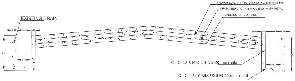
CROSS SECTION OF C. C ROAD
