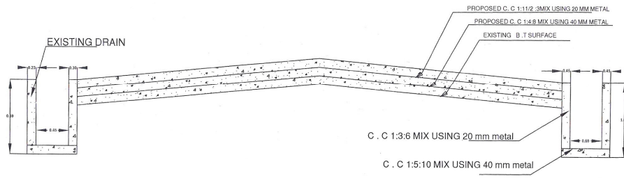
CROSS SECTION OF C . C ROAD
