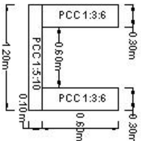
Cross Section of Drains
