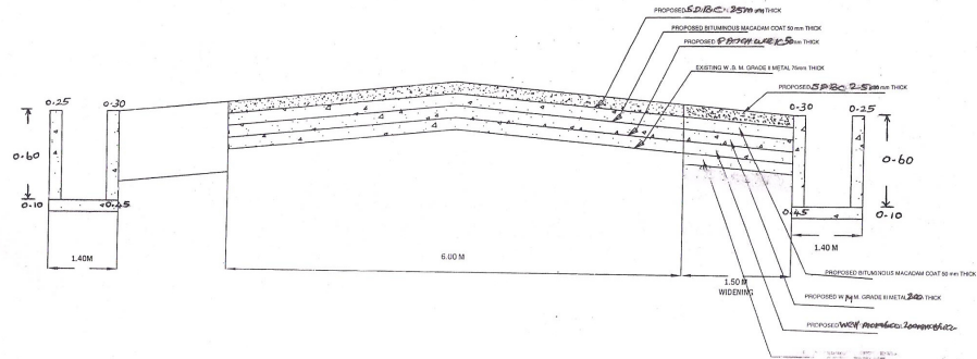
CROSS SECTION OF ROAD WITH DRAIN
