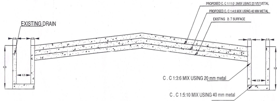
CROSS SECTION OF C . C ROAD
