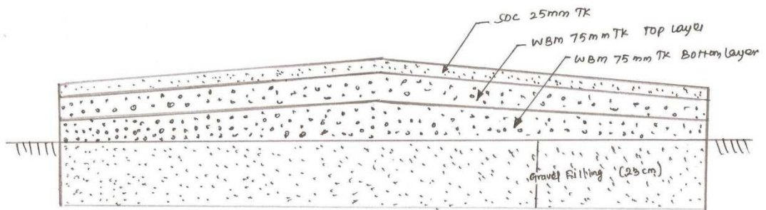
CROSS SECTION
