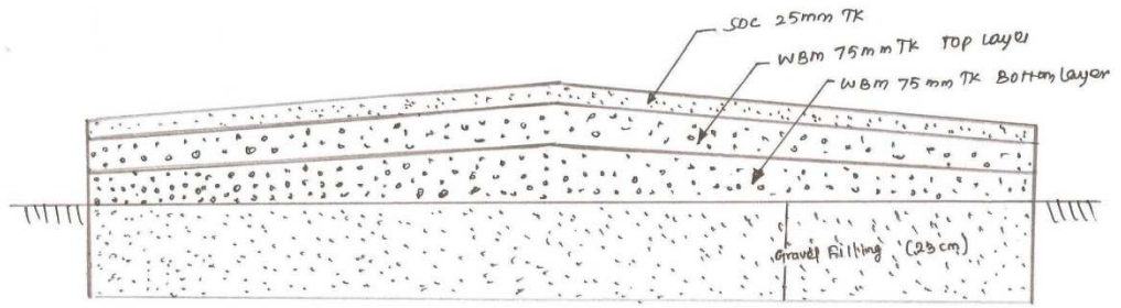
CROSS SECTION
