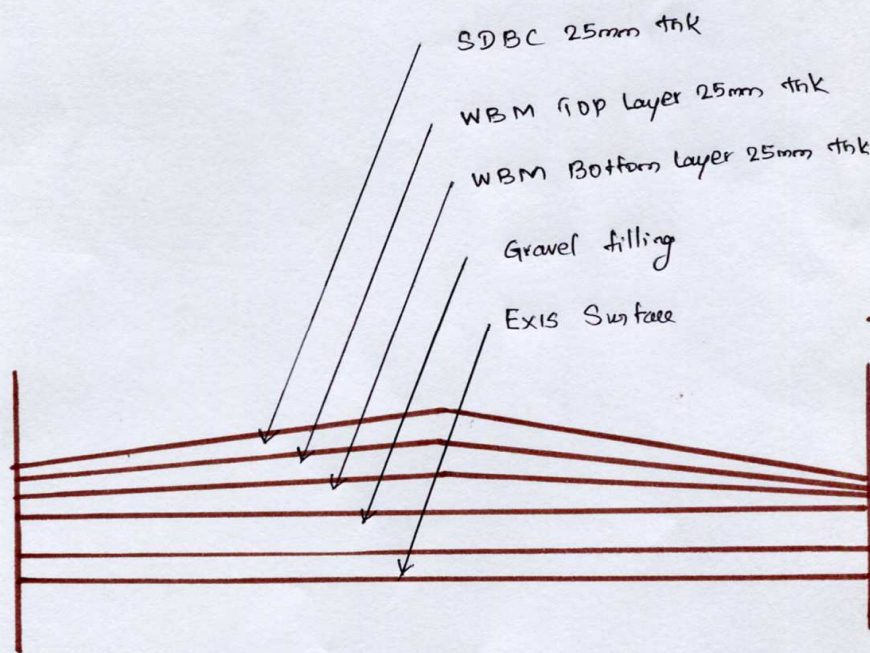
CROSS SECTION
