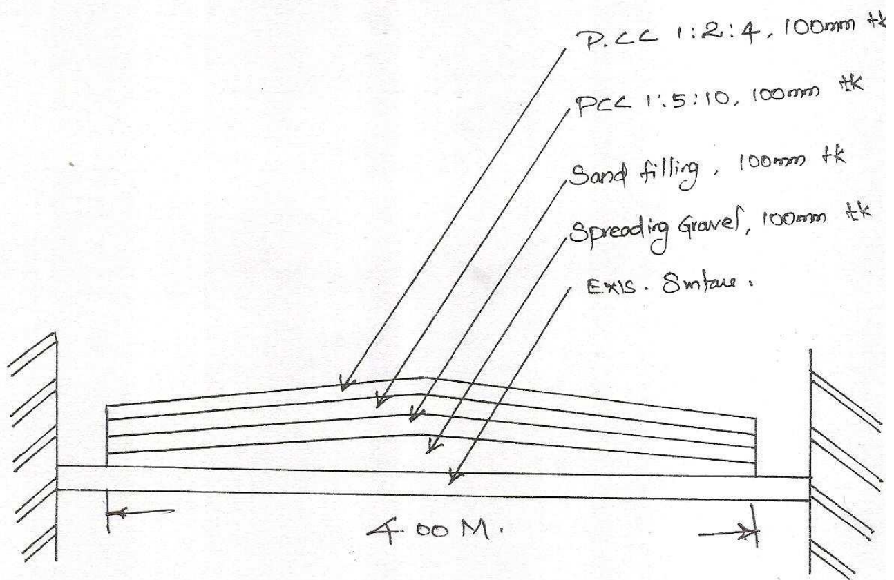
CROSS SECTION
