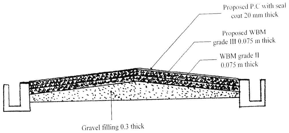
Cross section for Road work
