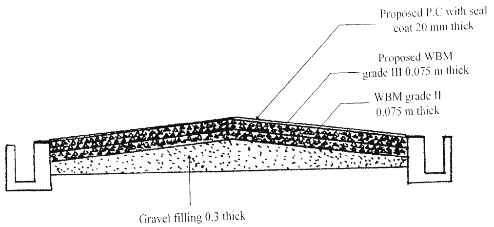
Cross section for Road work
