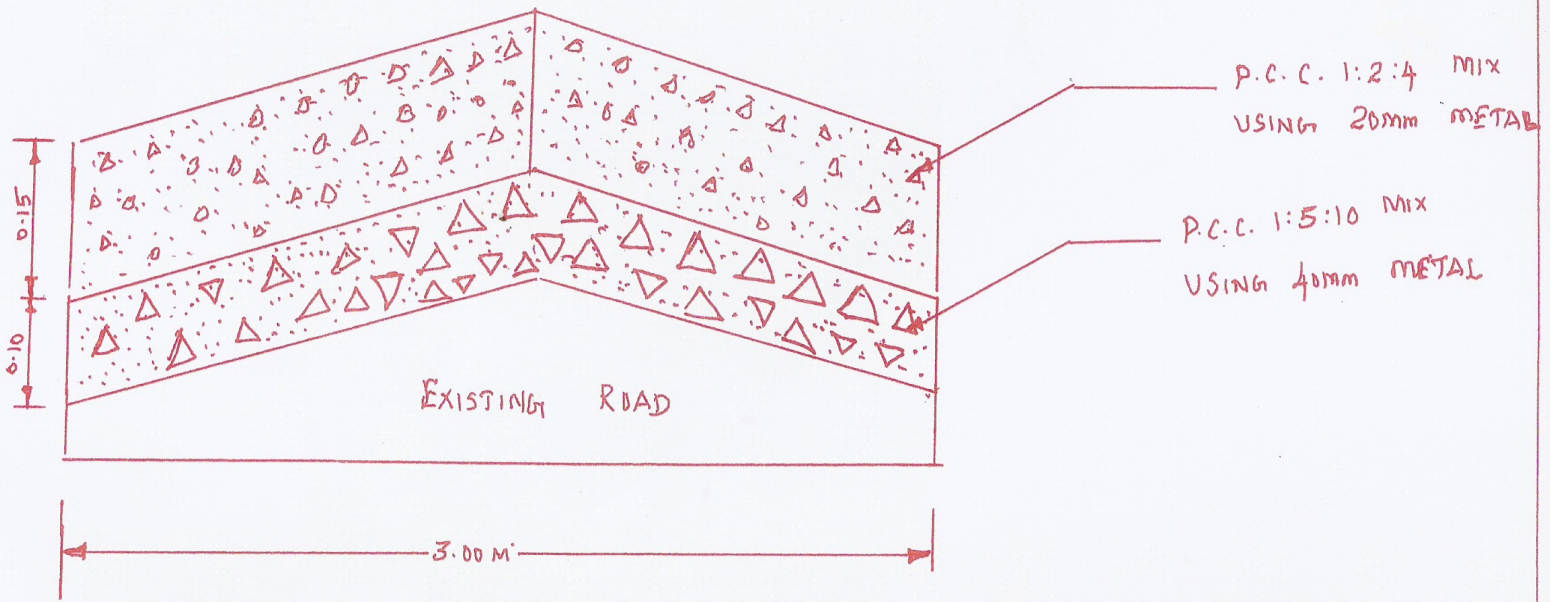
CROSS SECTION
