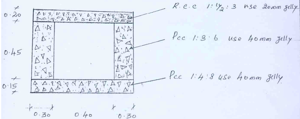
Cross section for Road work
