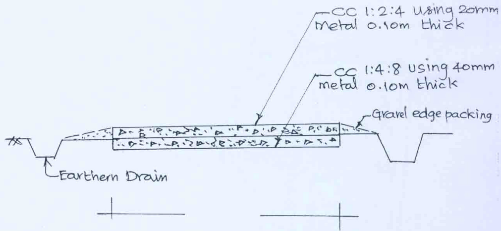
CROSS SECTION OF C.C. ROAD
