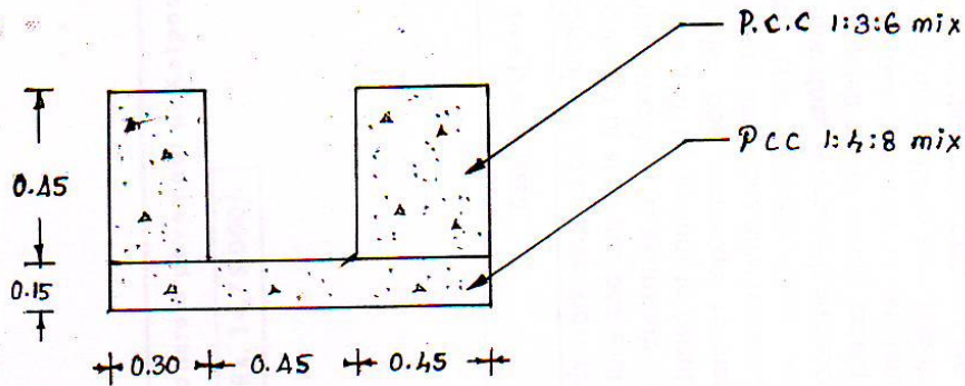
Section on Drainage
