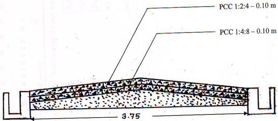
Cross section for Road work
