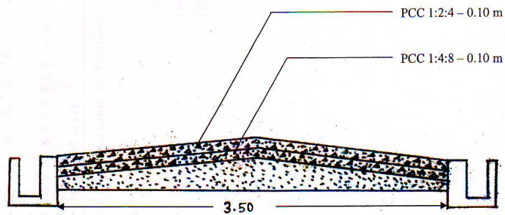
Cross section for Road work
