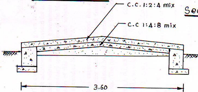
Section on Road
