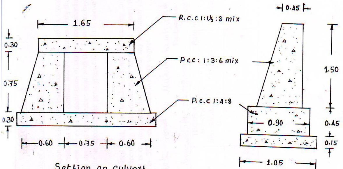
Section on culvert
