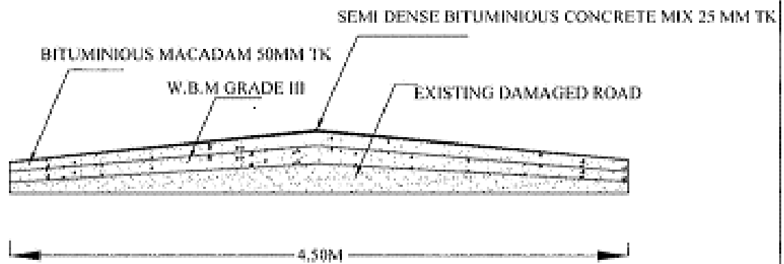
CROSS SECTION OF B.T ROAD
