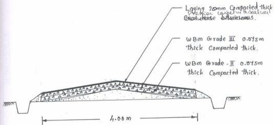
Cross Section on Road
