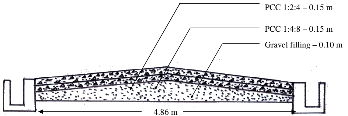
Cross section for Road work
