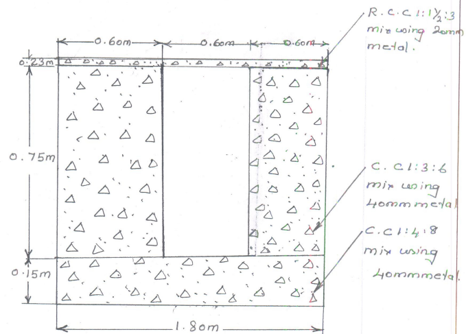
SECTION OF CULVERTE
