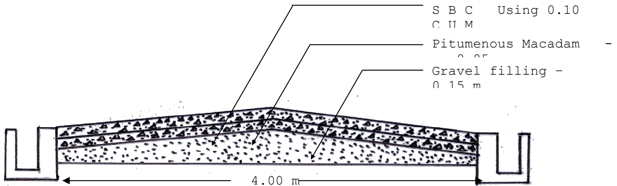
Cross section for Road work
