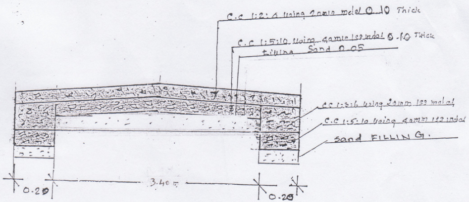
CROSS SECTION
