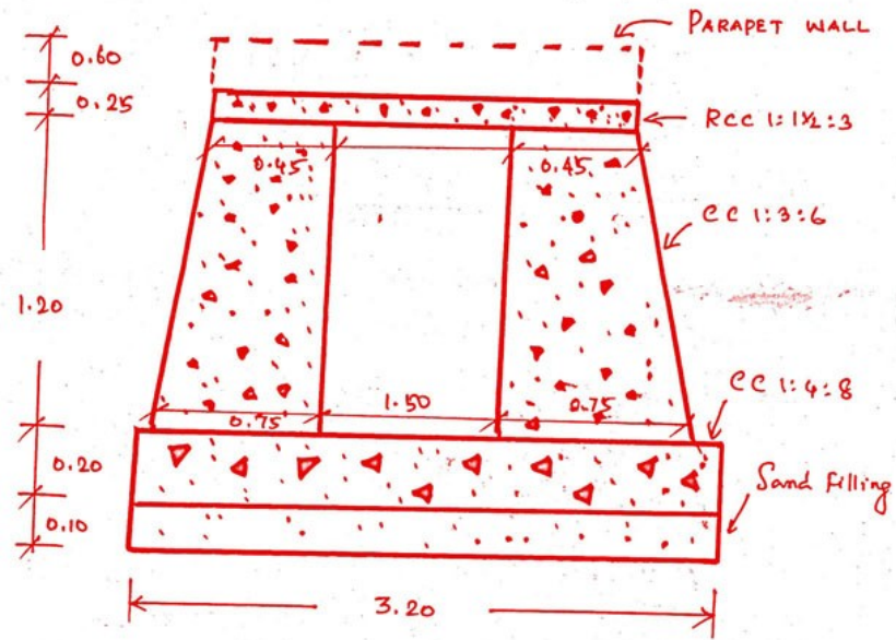
SECTION
