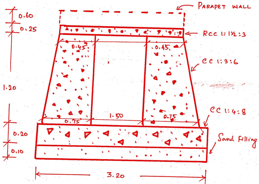
SECTION
