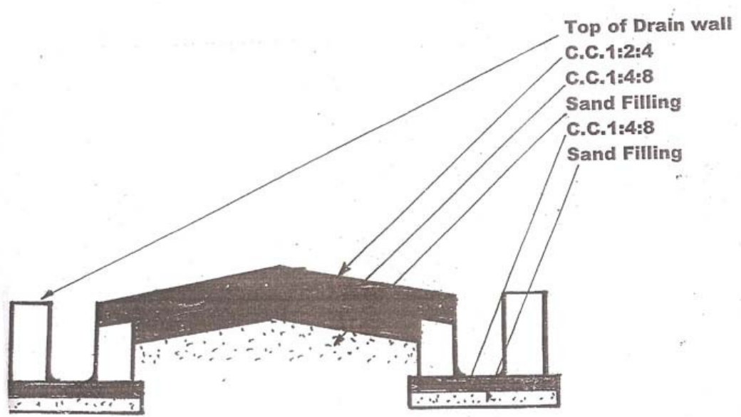
SECTION
