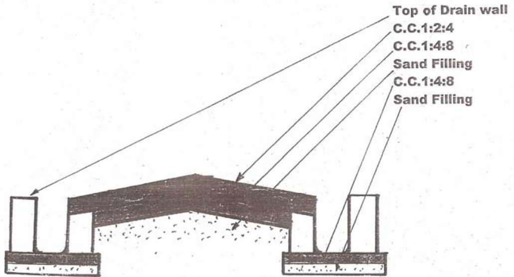
SECTION
