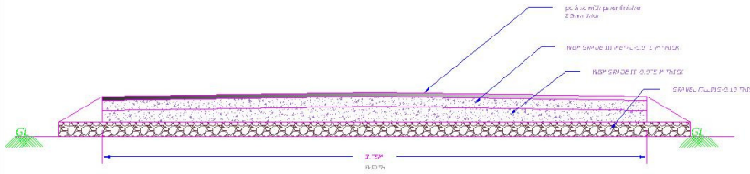
CROSS SECTION DOUBLE LAYER WBM WITH BT
