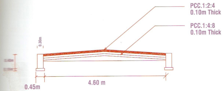
SECTION FOR CC. ROAD
