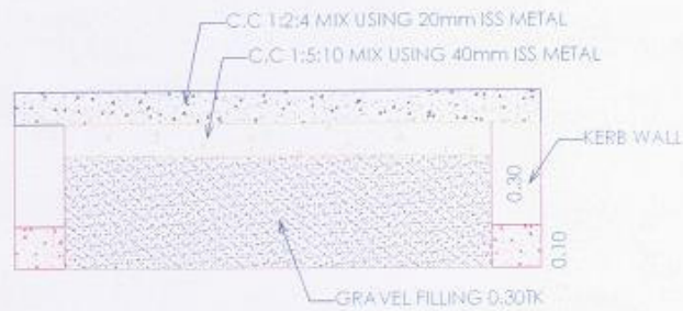
CROSS SECTION OF C.C.PAVEMENT
