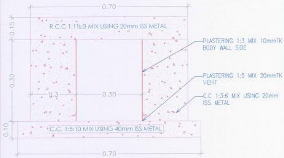
CROSS SECTION OF CULVERT
