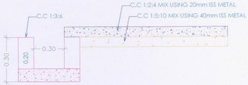
CROSS SECTION OF C.C PAVEMENT
