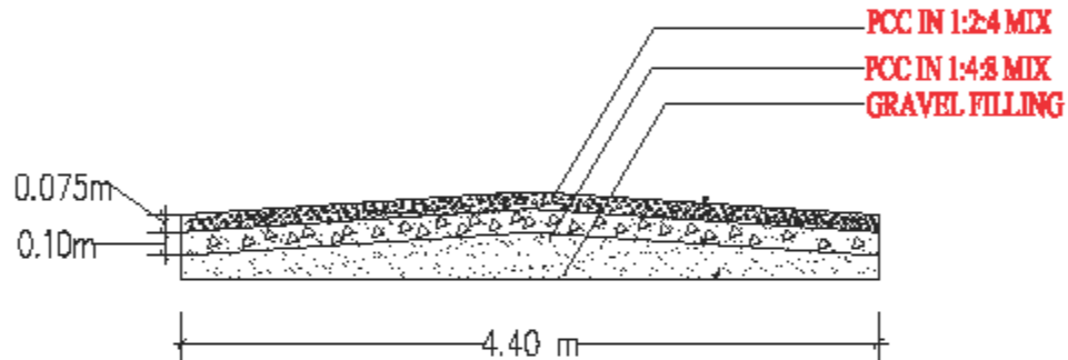
C.C ROAD CROSS SECTION
