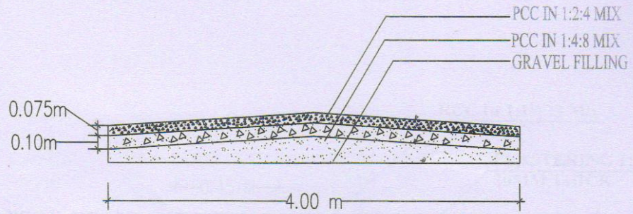
C.C ROAD CROSS SECTION
