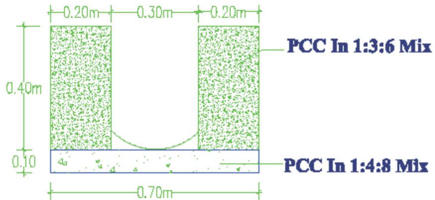
DRAIN CROSS SECTION
