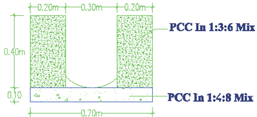
DRAIN CROSS SECTION
