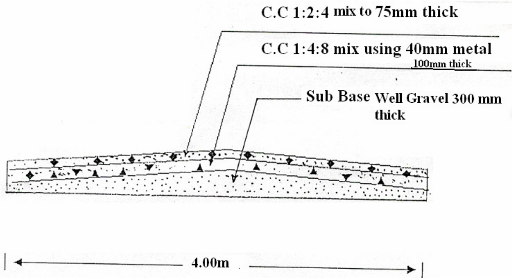
C.C Pavement - Cross Section
