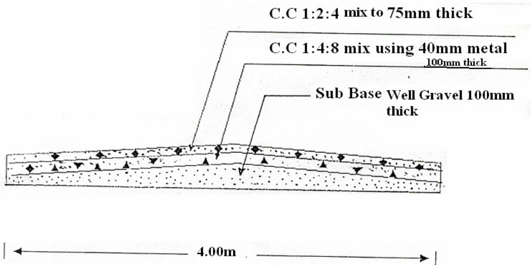
C.C Pavement - Cross Section
