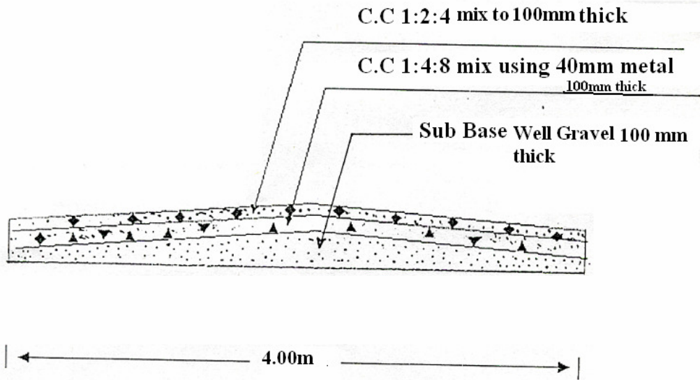
C.C Pavement - Cross Section
