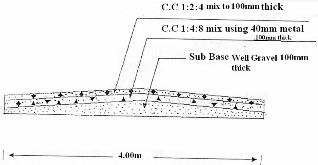
C.C Pavement - Cross Section
