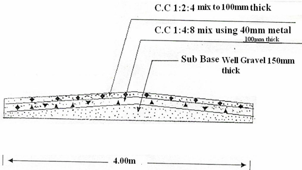
C.C Pavement - Cross Section
