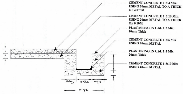
CROSS SECTION FOR DRAIN / CC ROAD
