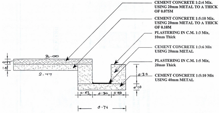
CROSS SECTION FOR C.C. ROAD ; GRAB.
