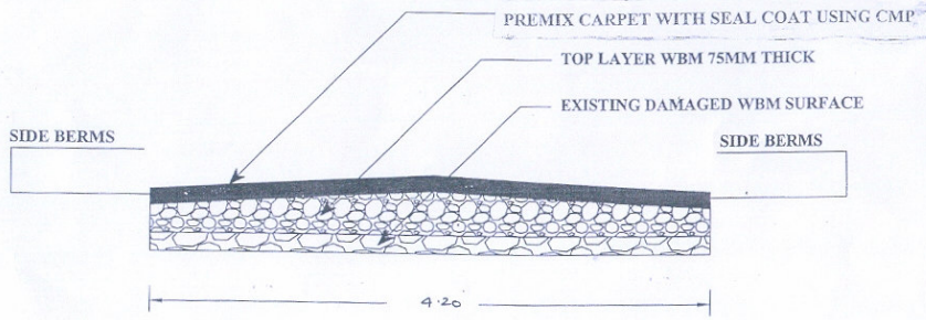
CROSS SECTION OF SINGLE LAYER WBM WITH BT
