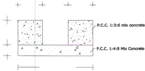
DRAIN CROSS SECTION
