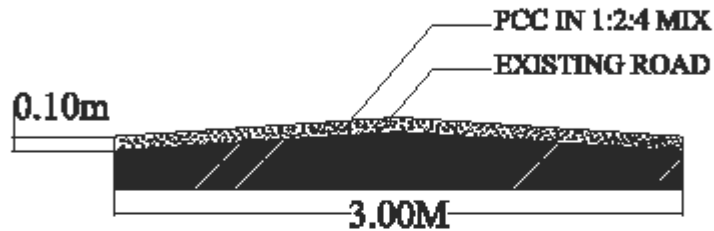
C.C ROAD CROSS SECTION
