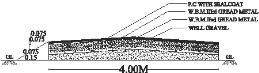
CROSS SECTION OF B.T ROAD
