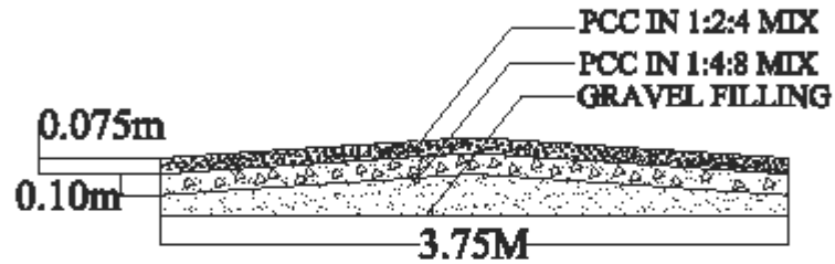
C.C. ROAD CROSS SECTION
