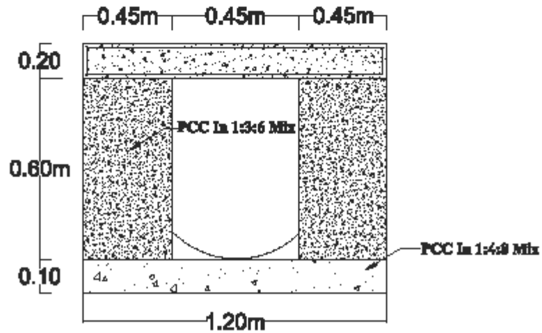
CALVERT CROSS SECTION
