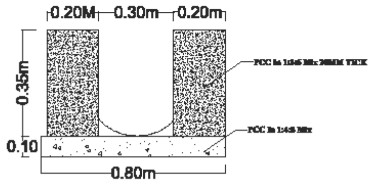
DRAIN CROSS SECTION
