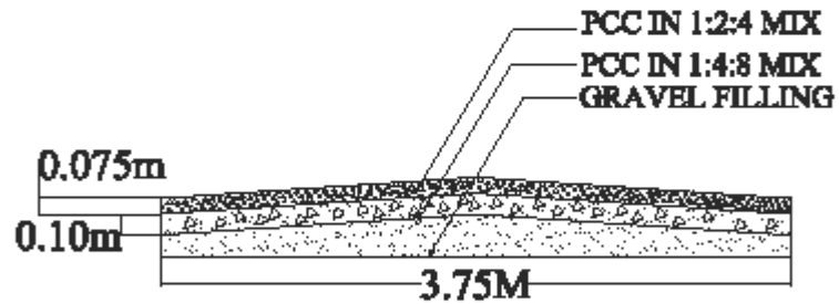
C.C ROAD CROSS SECTION
