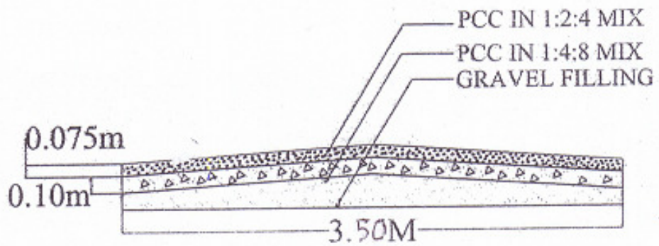
C.C ROAD CROSS SECTION
