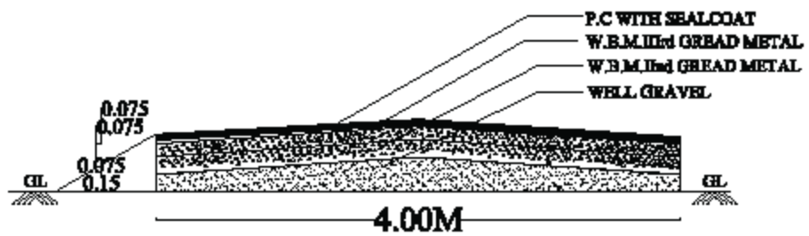
CROSS SECTION OF B.T ROAD
