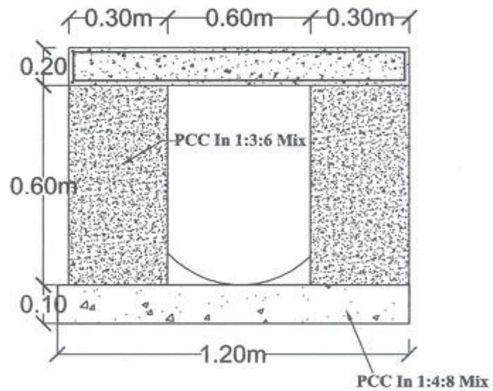
CALVERT CROSS SECTION
