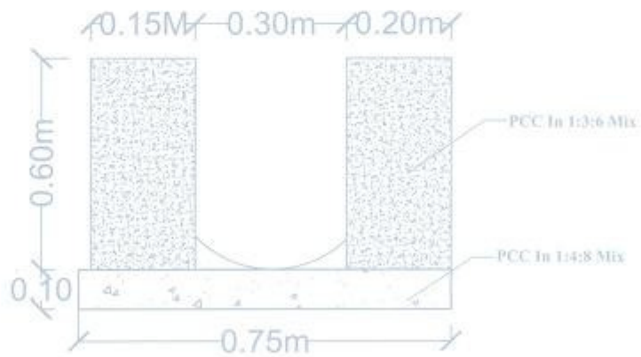
DRAIN CROSS SECTION
