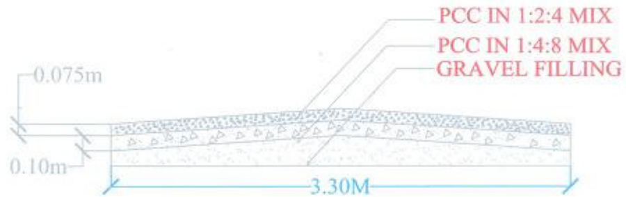
C.C ROAD CROSS SECTION
