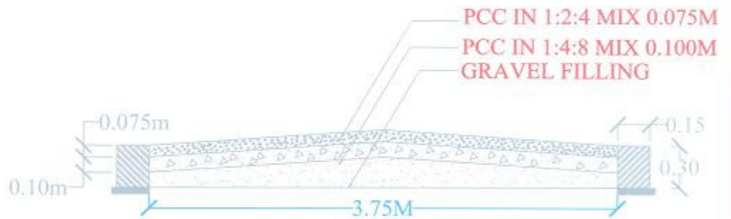
C.C ROAD CROSS SECTION
