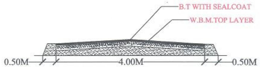
CROSS SECTION OF B.T ROAD
