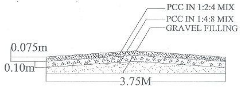
C.C ROAD CROSS SECTION
