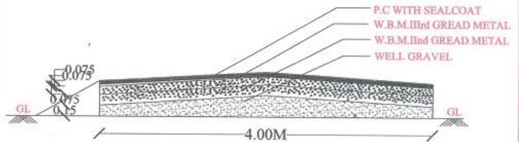
CROSS SECTION OF B.T ROAD
