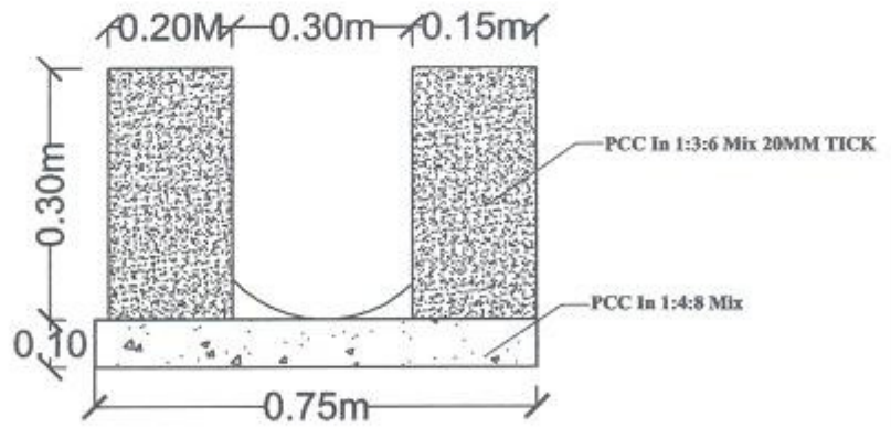
DRAIN CROSS SECTION
