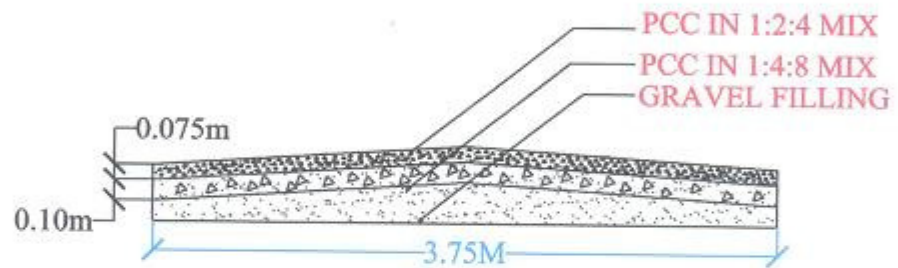
C.C ROAD CROSS SECTION
