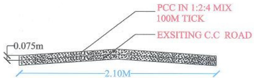
C.C ROAD CROSS SECTION
