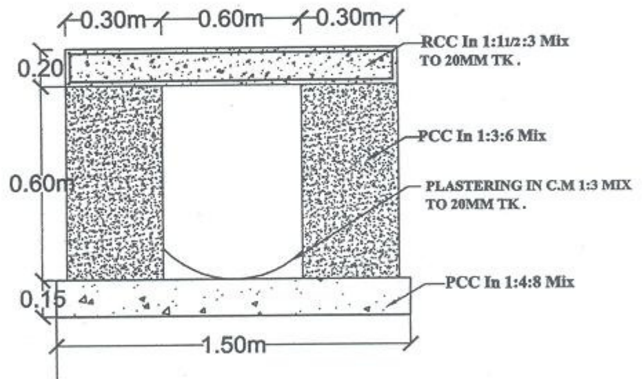
CULVERT CROSS SECTION
