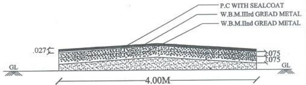
CROSS SECTION OF B.T ROAD
