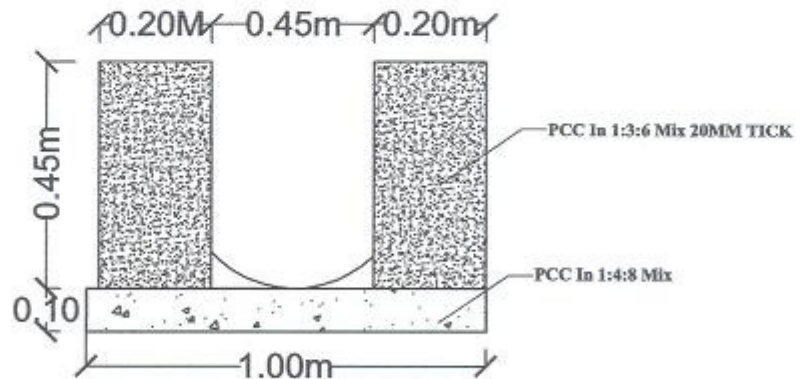
DRAIN CROSS SECTION
